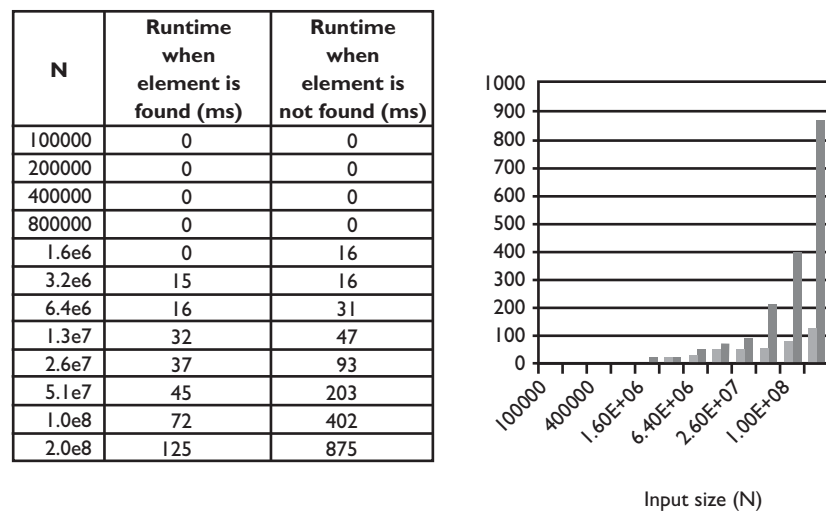
Figure 13.5 Runtimes for sequential search algorithm
