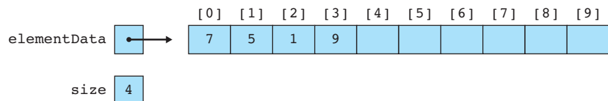
Figure 18.1 Representing a set as an unfilled, unsorted array
