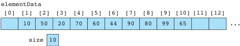
Figure 18.16 Heap implemented as array
