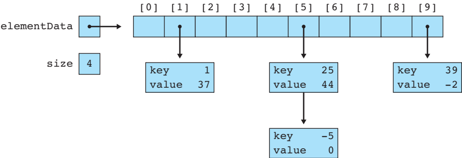
Figure 18.12 Hash map
