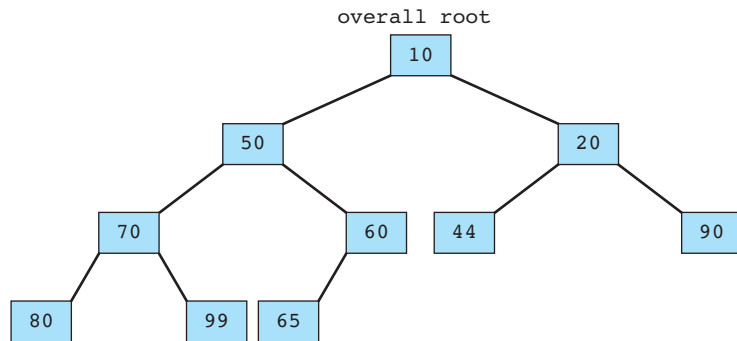
Figure 18.13 A min-heap
