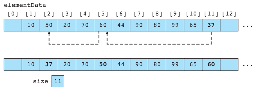
Figure 18.17 Array heap add operation
