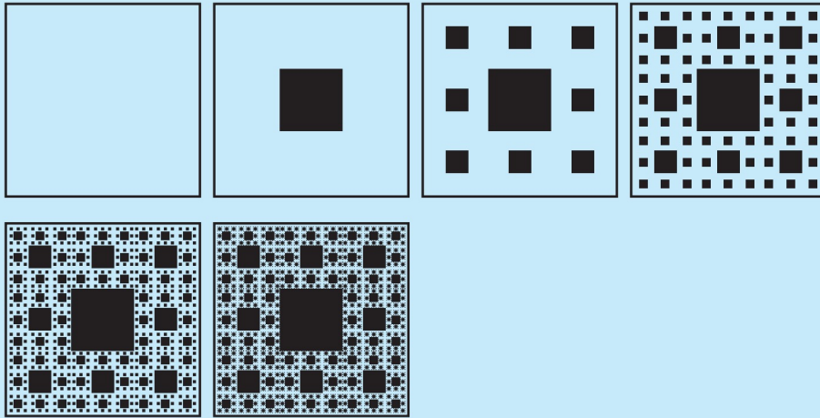
Figure 12.14 Sierpinski carpet
