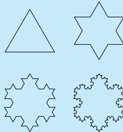
Figure 12.17 Koch snowflake
