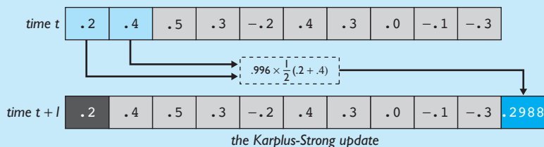
Figure 14.3 Karplus-Strong algorithm samples
