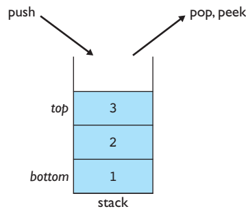
Figure 14.1 A stack
