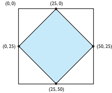
Figure 3G.12 Diamond
