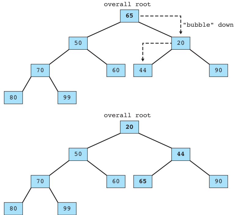
Figure 18.14 Removing from min-heap with bubble-down
