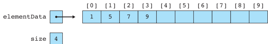
Figure 18.2 Representing a set as an unfilled, sorted array
