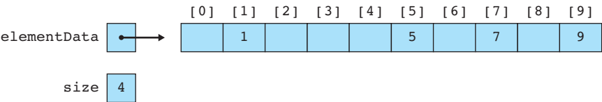
Figure 18.3 Storing set elements at corresponding indexes
