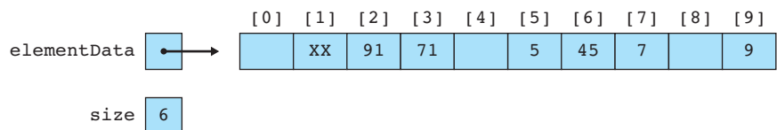
Figure 18.7 Removal of an element when probing is used
