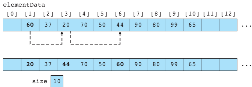
Figure 18.18 Array heap remove-min operation
