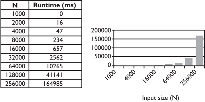
Figure 13.6 Runtimes for selection sort algorithm
