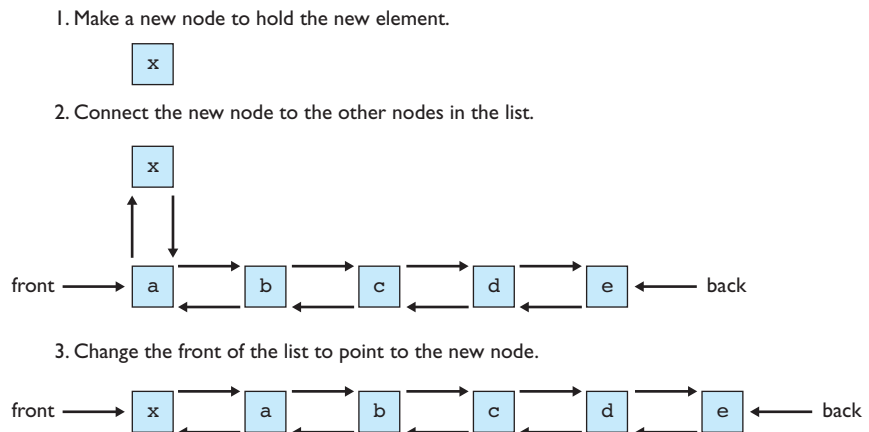
Figure 11.2 Adding an element to the front of a linked list
