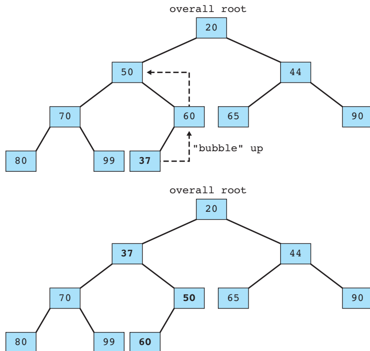
Figure 18.15 Adding to min-heap with bubble-up
